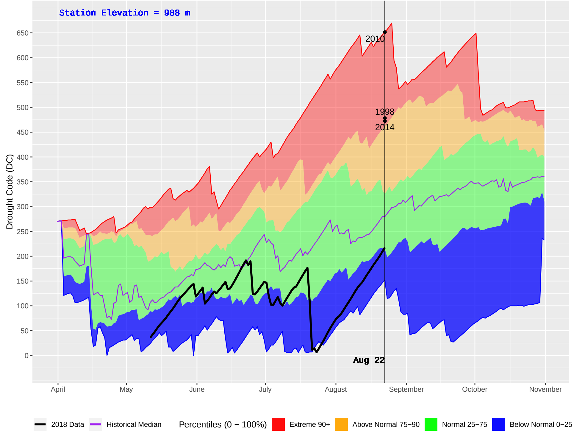
NOEL (437) : Historical (1993–2016) and Current (2018) Daily Drought Code (DC)
