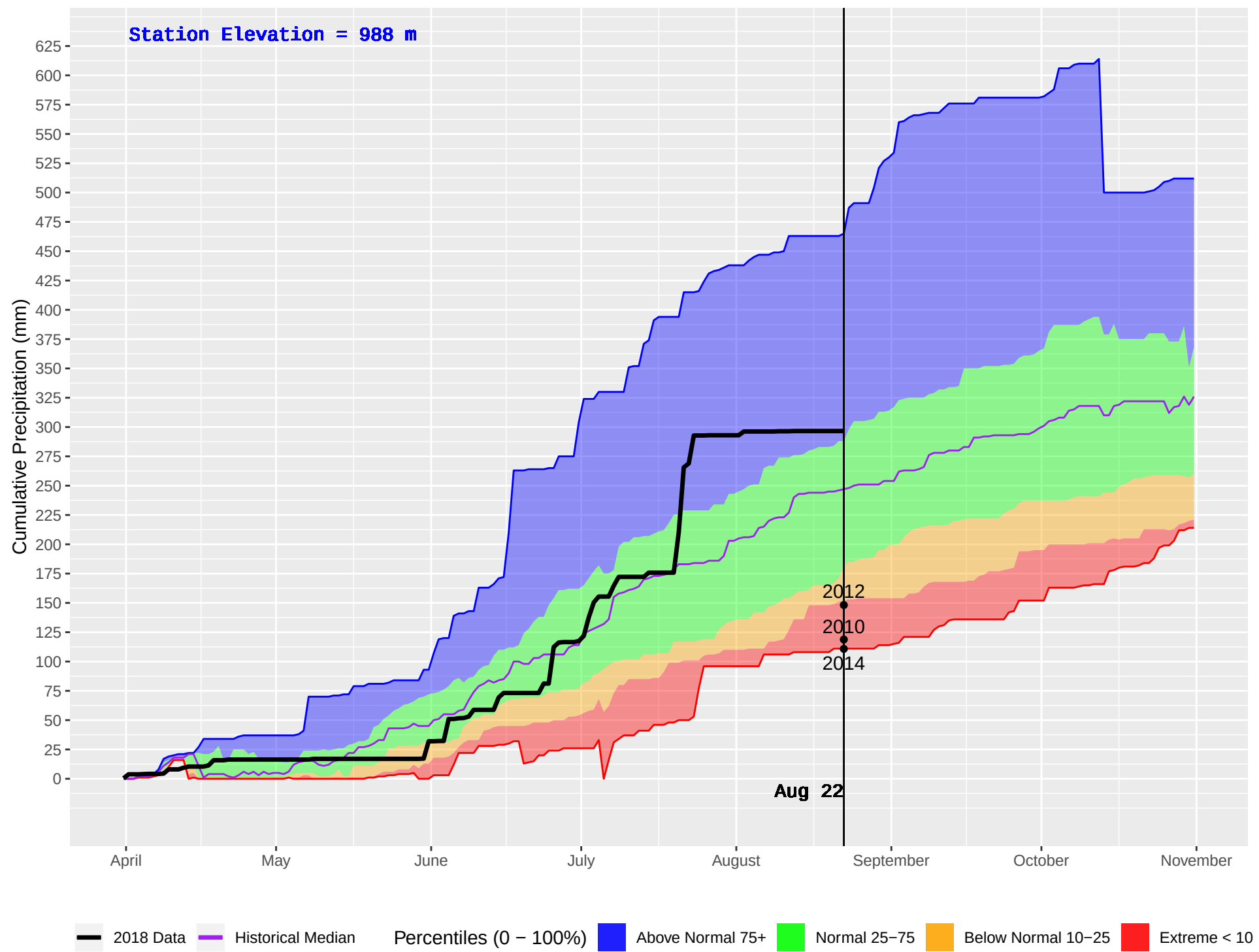
NOEL (437) : Historical (1993–2016) and Current (2018) Daily Cumulative Precipitation
