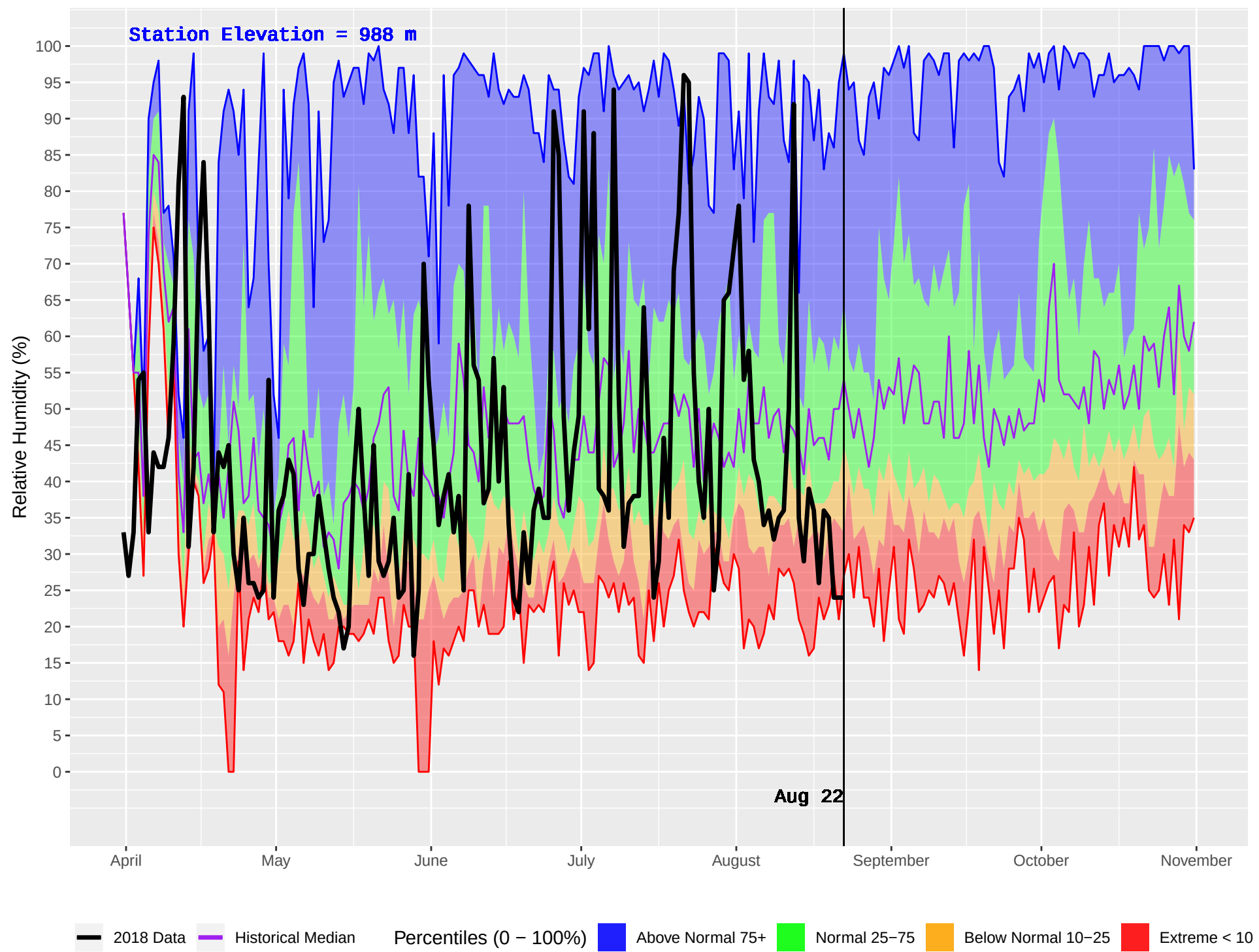
NOEL (437) : Historical (1993–2016) and Current (2018) Daily Relative Humidity
