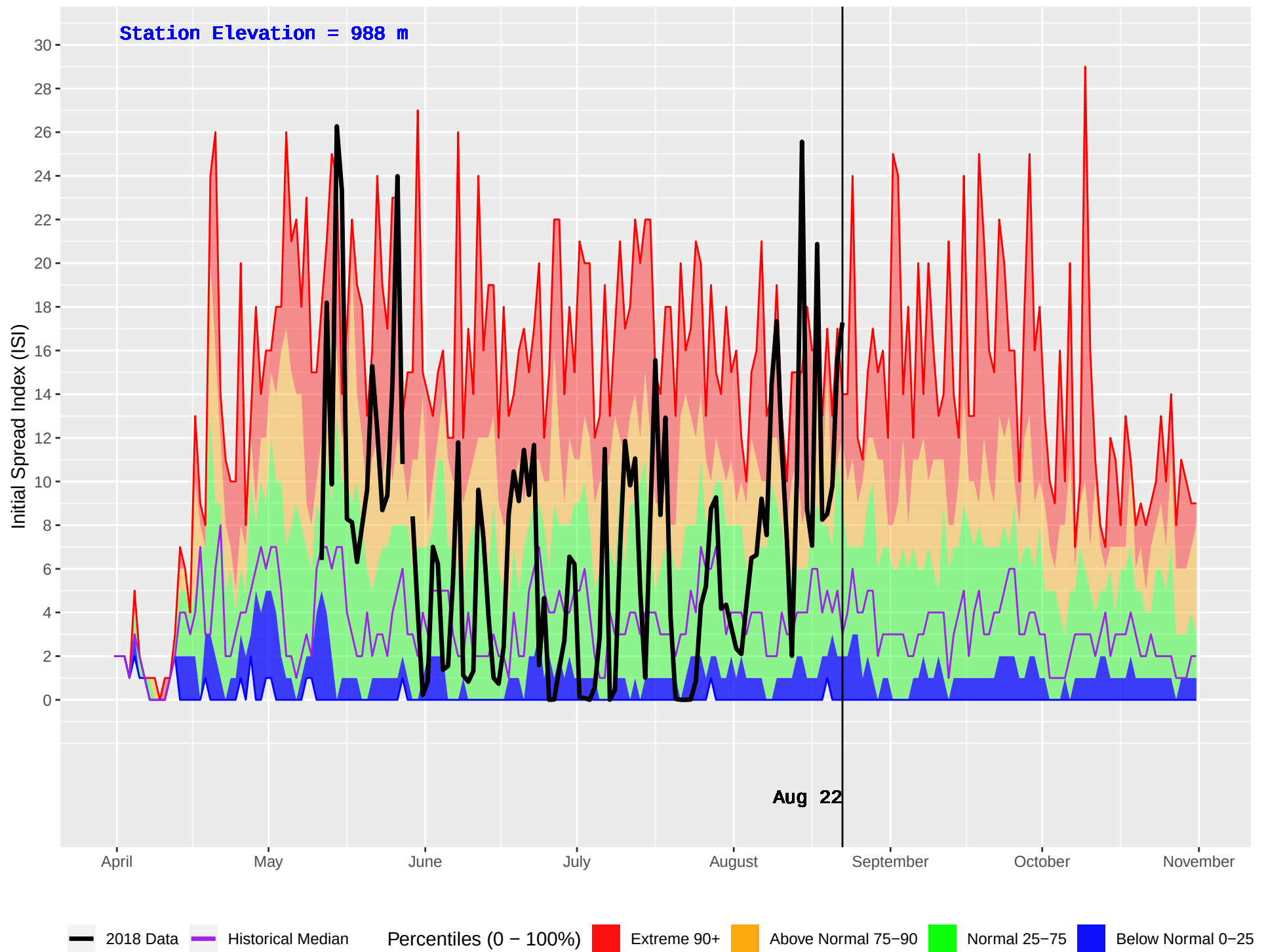
NOEL (437) : Historical (1993–2016) and Current (2018) Daily Initial Spread Index (ISI)
