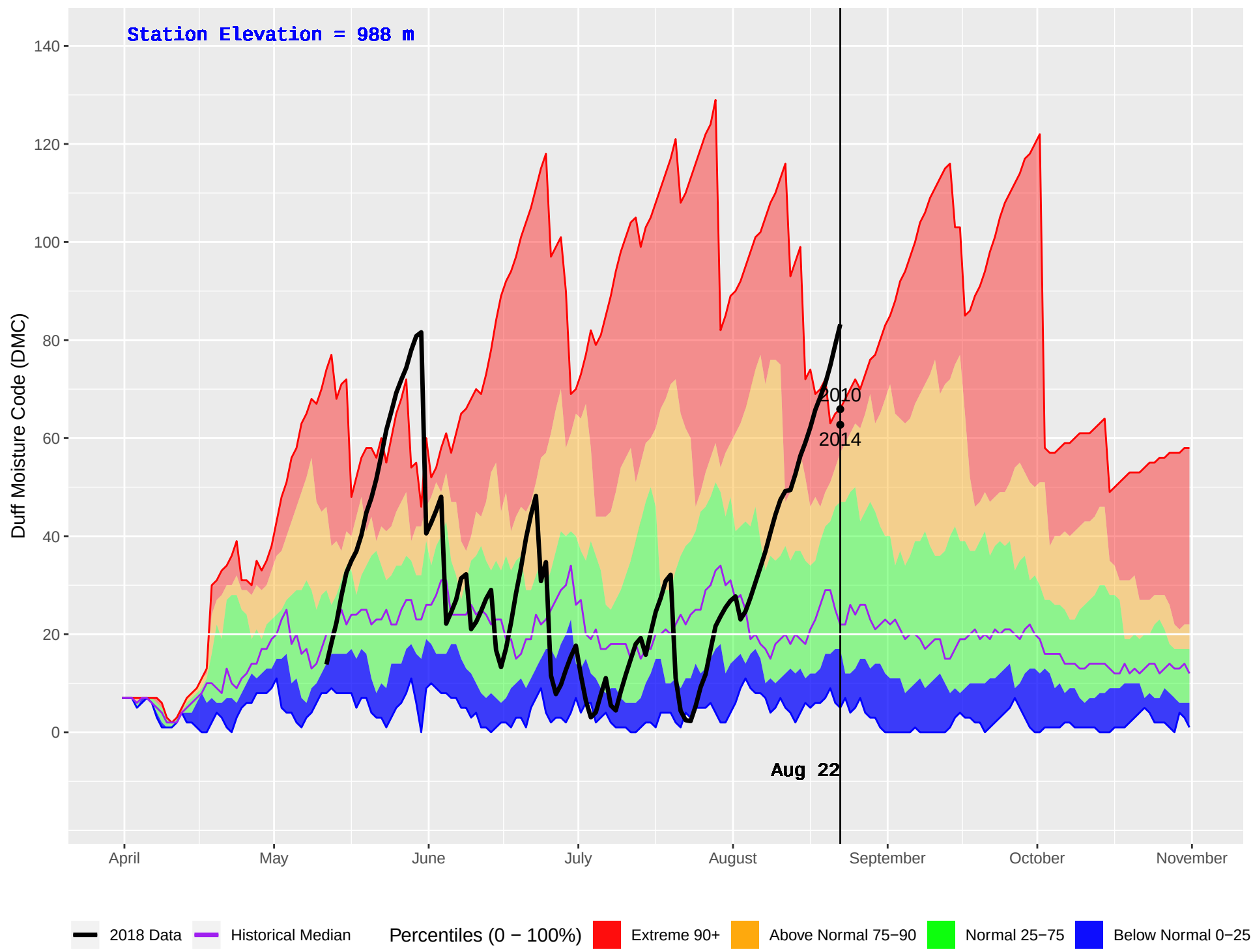
NOEL (437) : Historical (1993–2016) and Current (2018) Daily Duff Moisture Code (DMC)
