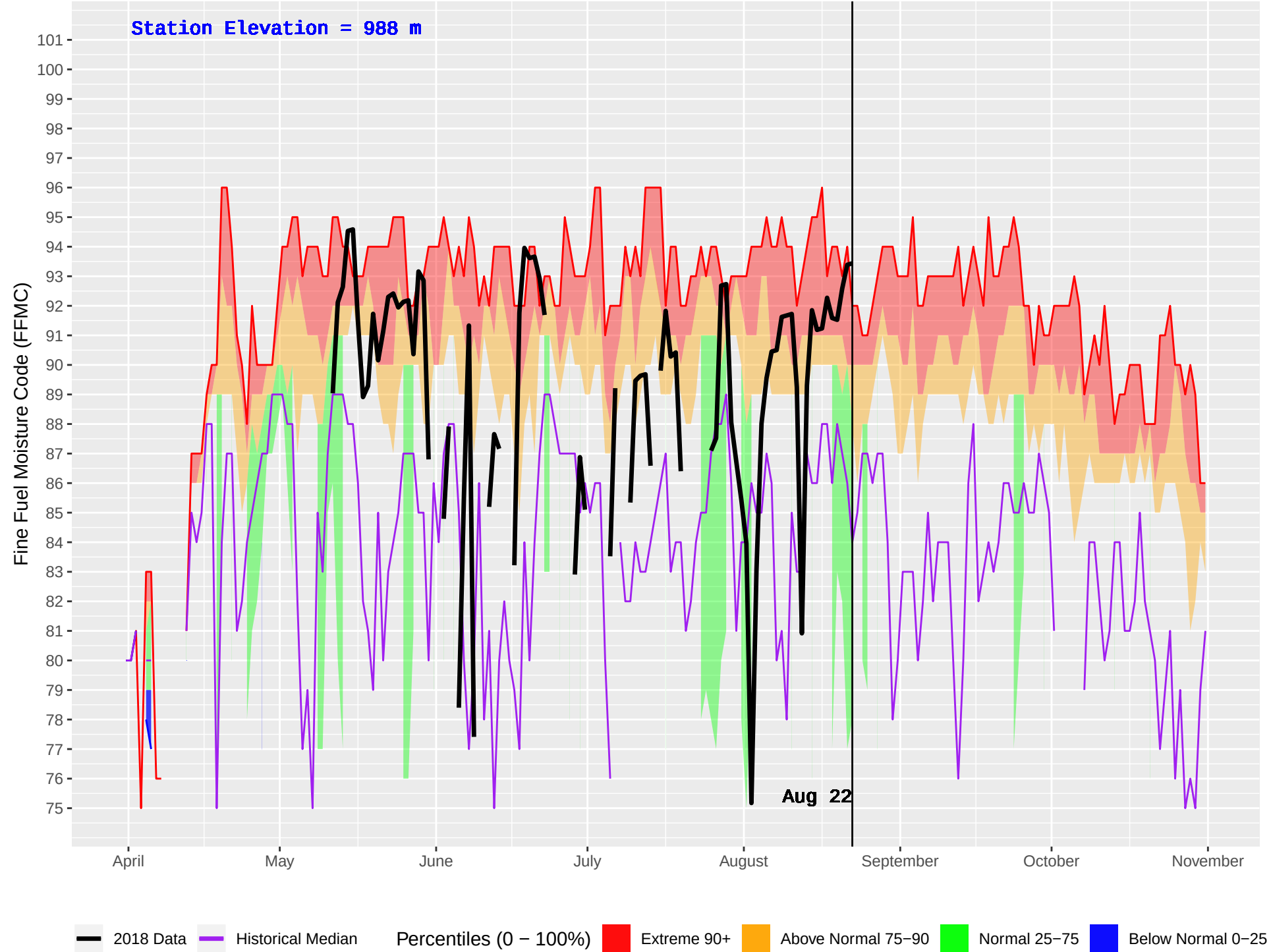
NOEL (437) : Historical (1993–2016) and Current (2018) Daily Fine Fuel Moisture Code (FFMC)
